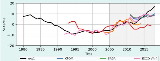
Figure 1: SLA time series of the run exp1, of altimetry products, and of the state estimate ECCO V4r4.
