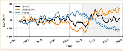
Figure 2: Monthly mean SLA time series with 12-month running mean.
